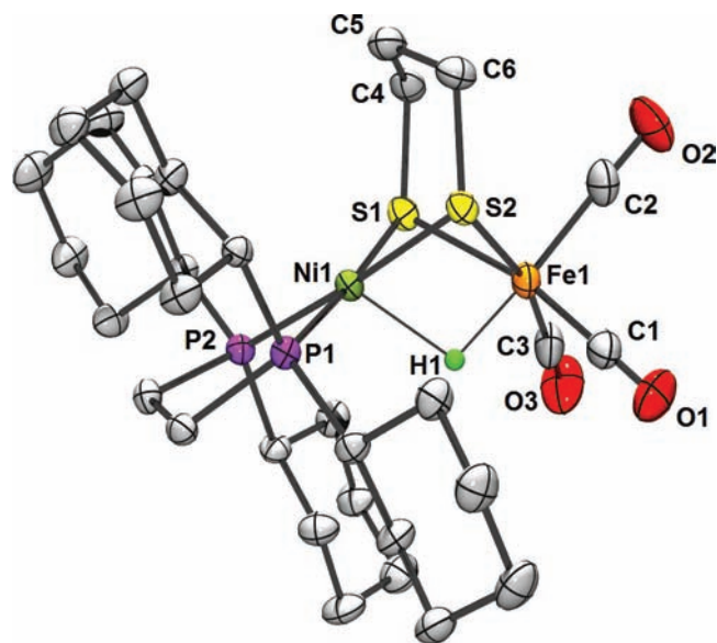
Figure 6. Molecular structure of the cation [\text{2H}]^+ in [\text{HNiFe}(\text{pdt})(\text{dcpe})(\text{CO})_3]\text{BF}_4 . Hydrogen (except the hydride ligand) atoms and \text{BF}_4^- are not shown. Selected distances ( \text{\AA} ): Ni–Fe, 2.6843(5); Ni–S(1), 2.2274(7); Ni–S(2), 2.2307(7); Fe–S(1), 2.3208(8); Fe–S(2), 2.3169(8); Ni–H, 1.90(2); Fe–H, 1.53(2).
