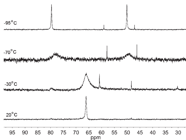
Figure 4. ^{31}\text{P}\{^1\text{H}\} NMR spectra of 3 (500 MHz, \text{THF-}d_8 solution) at various temperatures. The signal at \sim\delta 60 corresponds to \text{Ni}(\text{edt})\text{-(dppe)} , and the signal at \sim\delta 47 is unassigned.
