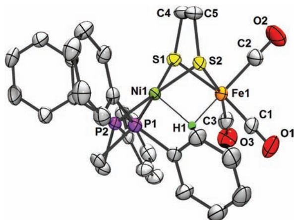
Figure 7. Molecular structure of the cation in [[\text{HNiFe}(\text{edt})(\text{dppe})(\text{CO})_3]^+ ( [\text{4H}]^+ ). Hydrogen (except the hydride ligand) atoms and \text{BF}_4^- are not shown. Selected distances (Å): Ni–Fe, 2.5958(6); Ni–S(1), 2.1969(9); Ni–S(2), 2.2128(9); Fe–S(1), 2.3152(9); Fe–S(2), 2.328(1); Ni–H, 1.84(3); Fe–H, 1.58(4).
