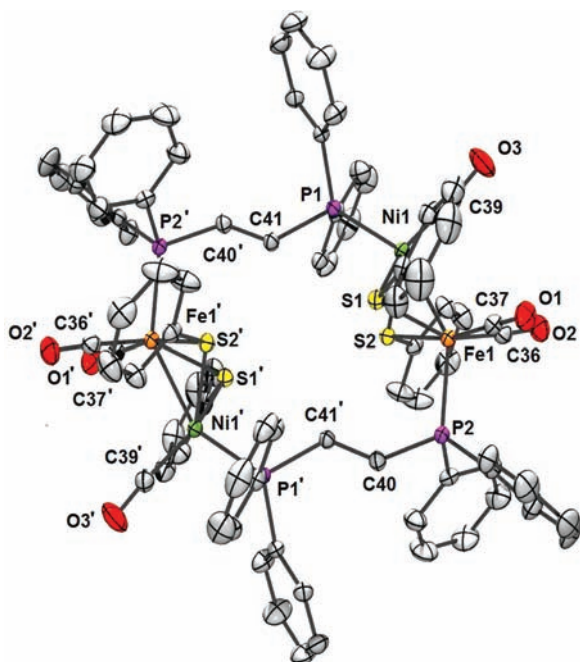
Figure 5. Structure of [(\text{CO})_2\text{Fe}(\text{SPh})_2\text{Ni}(\text{CO})_2(\mu\text{-dppe})_2] . Selected distances ( \text{\AA} ): Ni–Fe, 2.4567(3); Fe(1)–P(2), 2.2326(5); Ni(1)–P(1), 2.1905(5); Ni(1)–S(1), 2.2633(5); Ni(1)–S(2), 2.2784(5); Fe(1)–S(1), 2.2833(5); Fe(1)–S(2) 2.3167(6).
